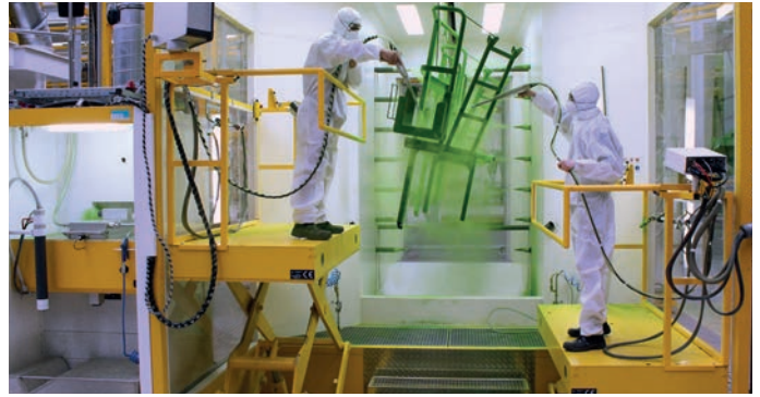
FCO Open Powder System - Fast colour change system designed for large and awkward shaped work pieces.
