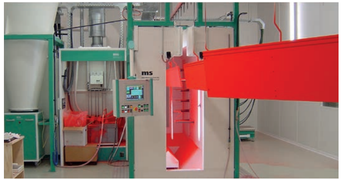
MDF Wood Coating - Complete coating and curing system with gas catalytic infrared oven.
