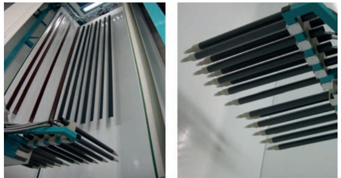
FCV Vertical Powder System - Vertical fast colour change system for profiles' coating.
